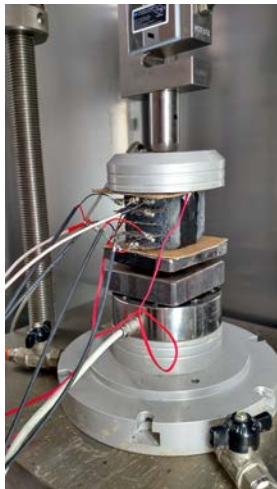
Dynamic testing of a strain-sensitive cement sample. Austin Downey
