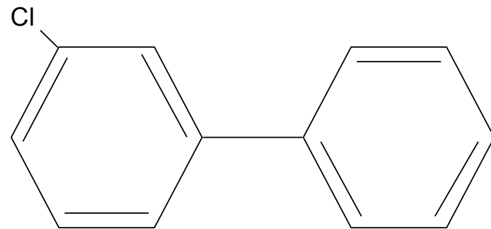
3-chlorobiphenyl
