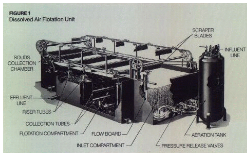
Dissolved air flotation (DAF) thickener
