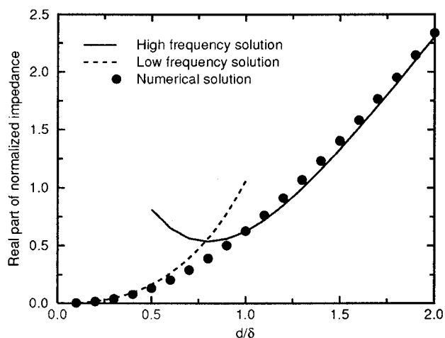
FIG. 4. Analytical and numerical solutions for the real part of the impedance change due to a long, surface-breaking crack.
