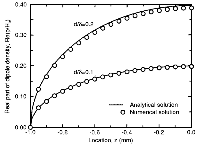
FIG. 1. Comparison between the real part of the analytical solution for the dipole density and the numerically calculated value for a long, surface-breaking crack in the low-frequency limit.
