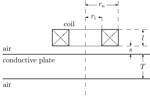
Figure 1. Cross-section through the axis of a circular, air-cored, eddy-current coil, positioned horizontally above a metal plate.
