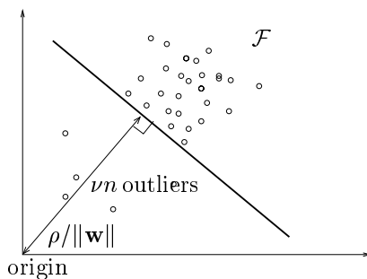
Fig. 12. Illustration of single-class idea. Solving Eq.(26), a hyperplane in \mathcal{F} is constructed that maximizes the distance to the origin while allowing for \nu outliers.
