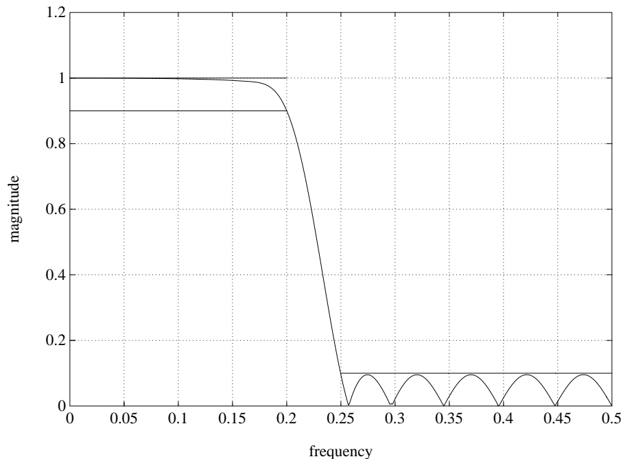
Figure 3. Flat Passband, Length-22, Minimum-Phase Filter.
