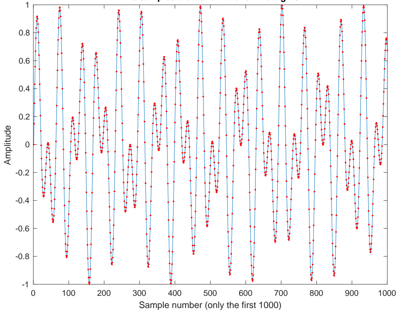
The sampled dial tone wave for the digit 5
