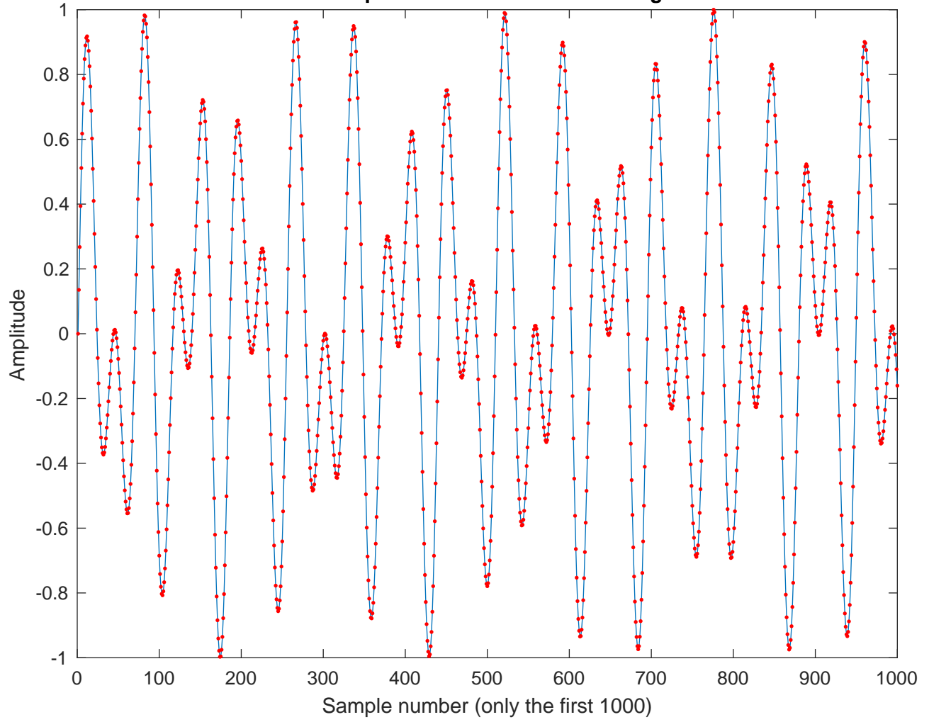
The sampled dial tone wave for the digit 1
