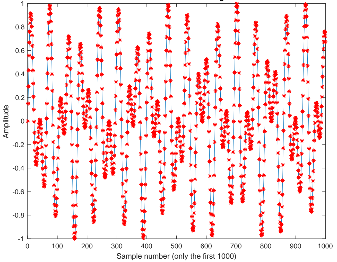
The dial tone wave for the digit 5
