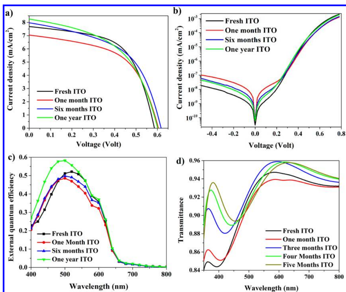
Figure 3. Current–voltage characteristics of P3HT:PC 60 BM OPVs (a) under illumination and (b) in the dark. (c) External quantum efficiency of P3HT:PC 60 BM OPVs. Shown current–voltage and quantum efficiency curves were from a single cell on a substrate containing six cells in total. Averages of all cells are presented in Table 2. (d) Optical transmission of fresh and old ITO substrates without any device layer.
