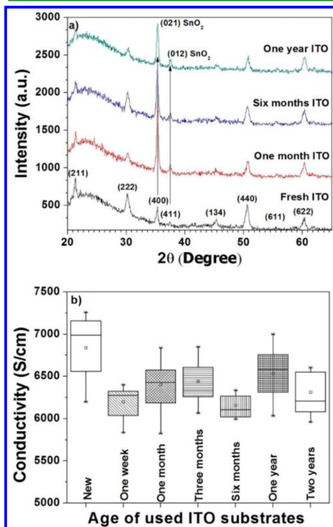
Figure 1. (a) X-ray diffraction spectra of fresh, 1-month-old, 6-month-old, and 1-year-old ITOs. (b) Conductivity boxplots of more than 30 old ITO substrates of different ages.
