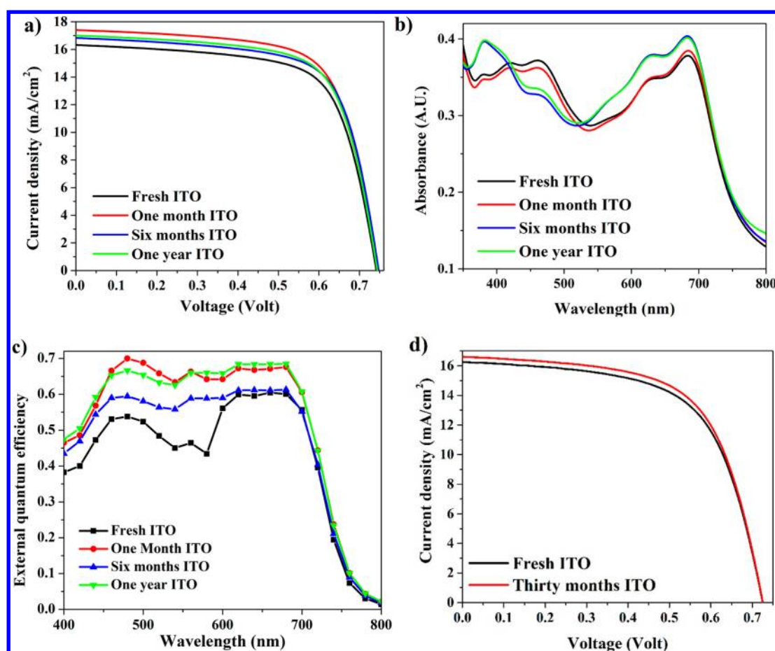
Figure 4. (a) Current–voltage characteristics of PTB7:PC 70 BM OPV devices under illumination, (b) absorbance of ITO/PEDOT:PSS/PTB7:PC 70 BM structures, and (c) external quantum efficiency of PTB7:PC 70 BM devices. Shown current–voltage and quantum efficiency curves were from a single cell on a substrate containing six cells in total. Averages of all cells are presented in Table 2. (d) Current–voltage characteristics of PTB7:PC 70 BM devices on the fresh and oldest ITO tested in this study.
