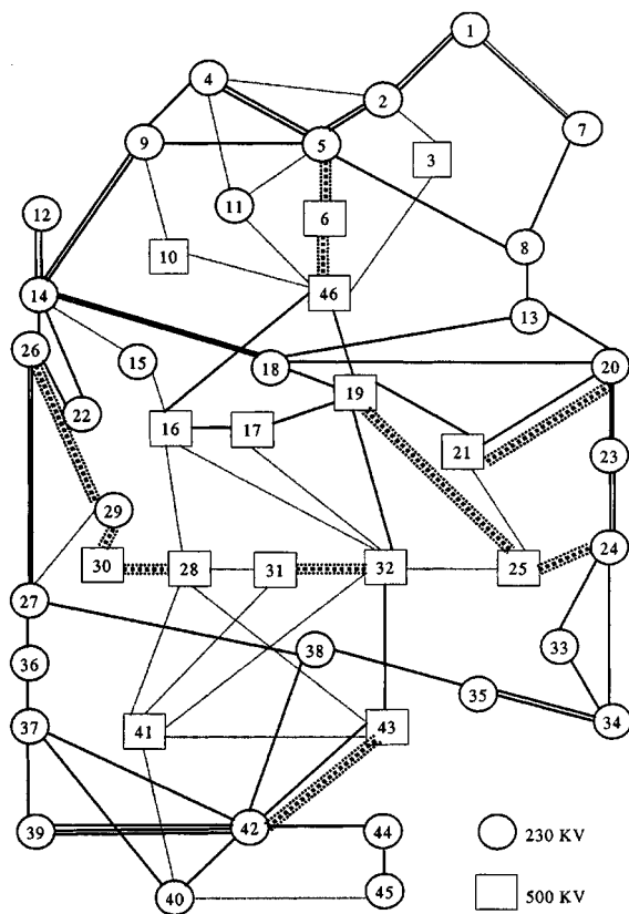
Fig. 1. 46 bus network and solution (without redispatch).
