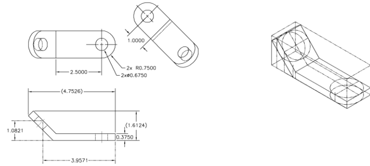
Isometric Construction Demo
