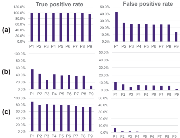
Figure 3: Accuracy comparisons between different parameter sets and mathematical models. (a) Linear regression; (b) logistic regression; (c) SVM classifier.
