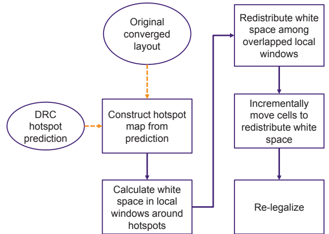
Figure 5: The predictor-guided routability optimization algorithm.
