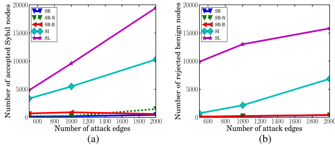
Fig. 8. The number of accepted Sybil nodes and rejected benign nodes as a function of the number of attack edges. The benign region is the Facebook network, and the Sybil regions are synthesized by PA model. We observe that SB, SB-N, and SB-B all work an order of magnitude better than previous classification systems. Furthermore, we find that incorporating both benign and Sybil labels increases the performance of our algorithm. (a) Accepted Sybil nodes. (b) Rejected benign nodes.
