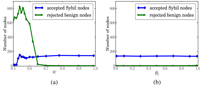
Fig. 4. The number of accepted Sybil nodes and rejected benign nodes as a function of the model parameters w and \theta_l . (a) \theta_l = 0.50 and we vary w . (b) w = 0.90 and we vary \theta_l . We observe that there exists a phase transition point w_0 (e.g., w_0 \approx 0.65 in our experiments) for the parameter w . SybilBelief is robust for w > w_0 . Moreover, we confirm that SybilBelief performance is independent with \theta_l once it's bigger than 0.
